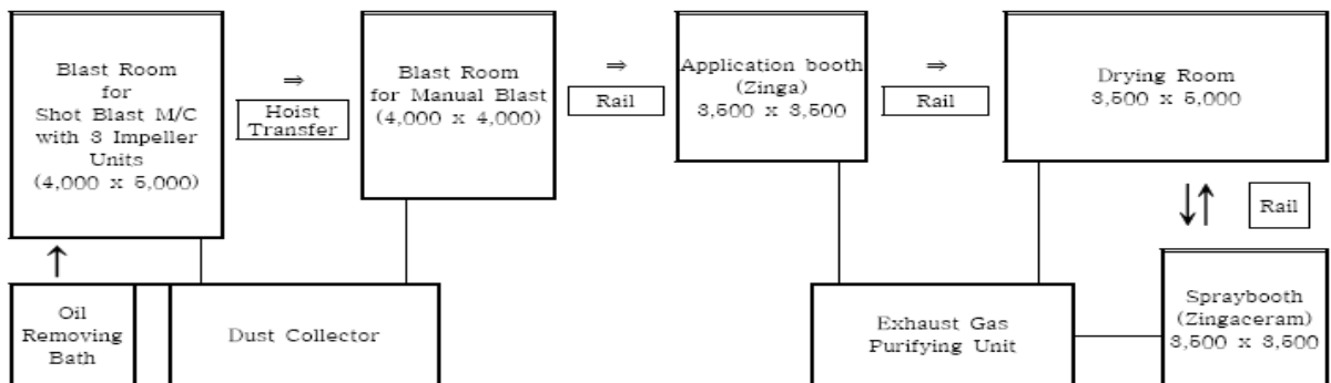
* Shop Layout for Zinga Application on Transformers
